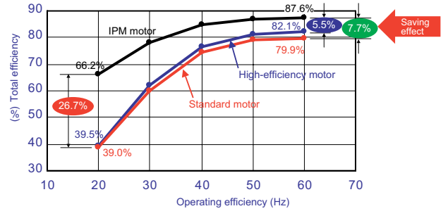
• Characteristics of frequency - total efficiency (example of 400V, 3.7kW)
